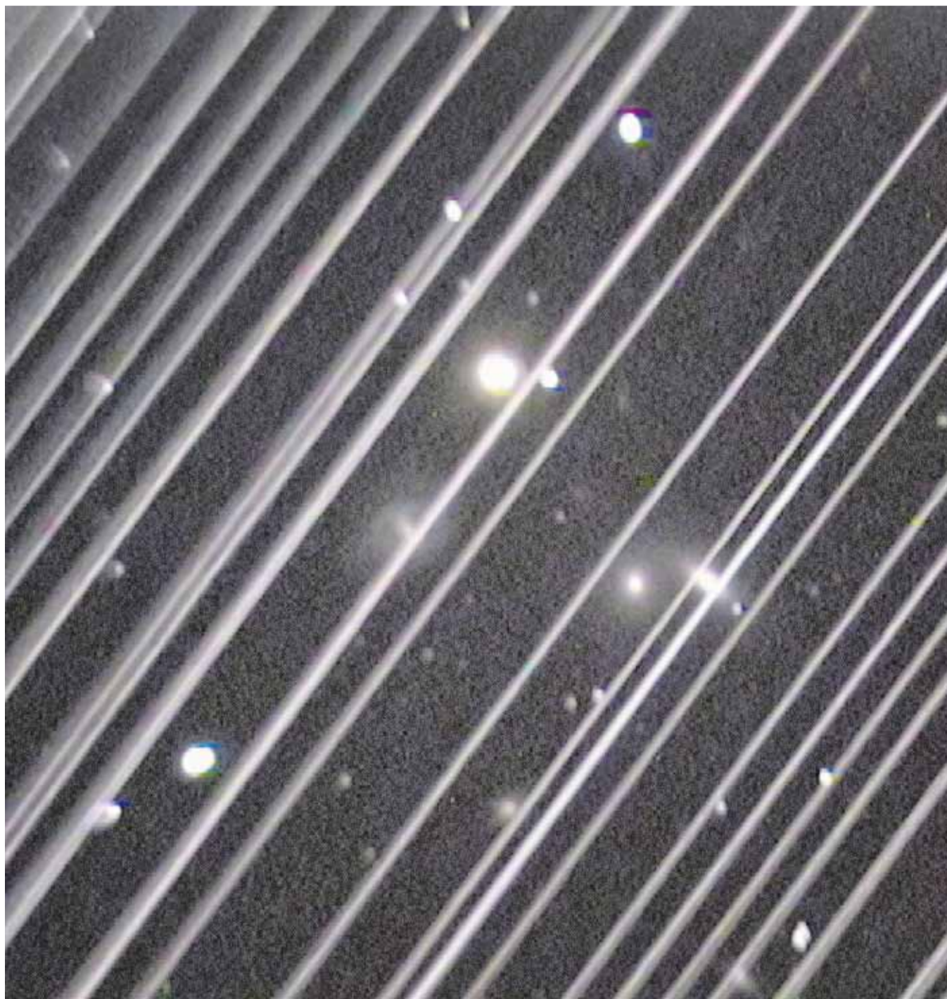
VICTORIA GIRGIS / LOWELL OBSERVATORY
